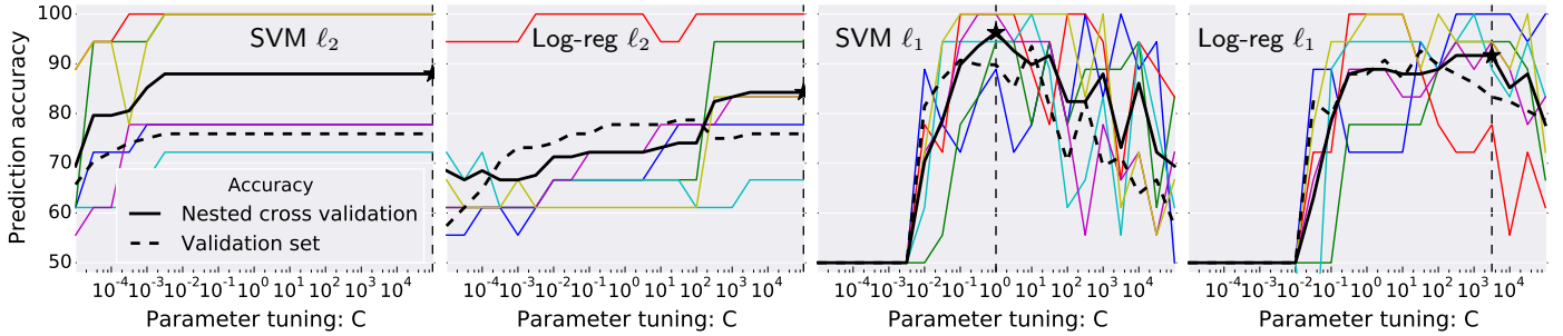
Figure 8: Tuning curves for SVM \ell_2 , logistic regression \ell_2 , SVM \ell_1 , and logistic regression \ell_1 , on the scissors / scramble discrimination for the Haxby dataset [16]. The thin colored lines are test scores for each of the internal cross-validation folds, the thick black line is the average of these test scores on all folds, and the thick dashed line is the score on left-out validation data. The vertical dashed line is the parameter selected on the inner cross-validation score.
