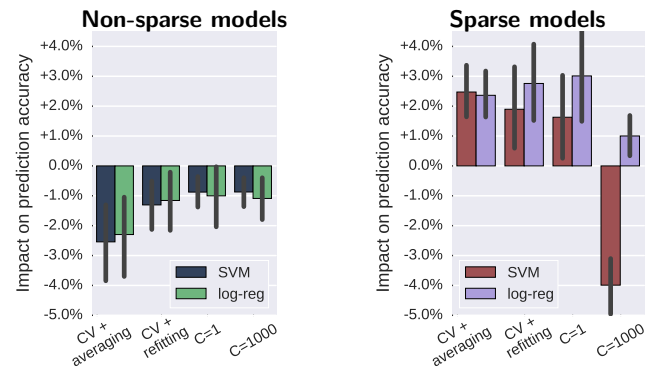
Figure 9: Prediction accuracy: impact of the parameter-tuning strategy. For each strategy, difference to the mean prediction accuracy in a given validation split.
