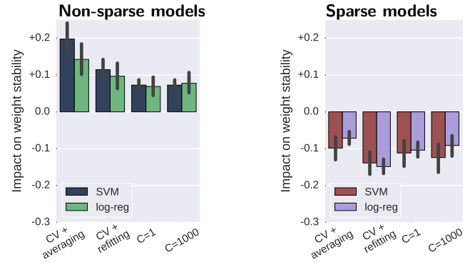
Figure A6: Impact of the parameter-tuning strategy on stability of weights without feature standardization: for each strategy, difference to the mean stability of the model weights across validation splits.
