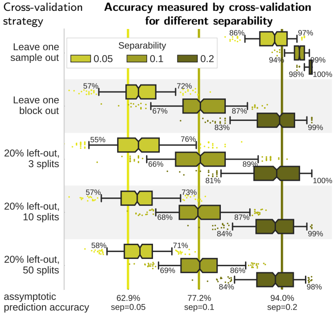
Figure A2: Cross-validation measures on simulations. Prediction accuracy, as measured by cross-validation (box plots) and on a very large test set (vertical lines) for different separability on the simulated data and for different cross-validation strategies: leave one sample out, leave one block of samples out (where the block is the natural unit of the experiment: subject or session), or random splits leaving out 20% of the blocks as test data, with 3, 10, or 50 random splits. The box gives the quartiles, while the whiskers give the 5 and 95 percentiles. Note that here leave-one-block-out is similar of 10 splits of 10% of the data.
