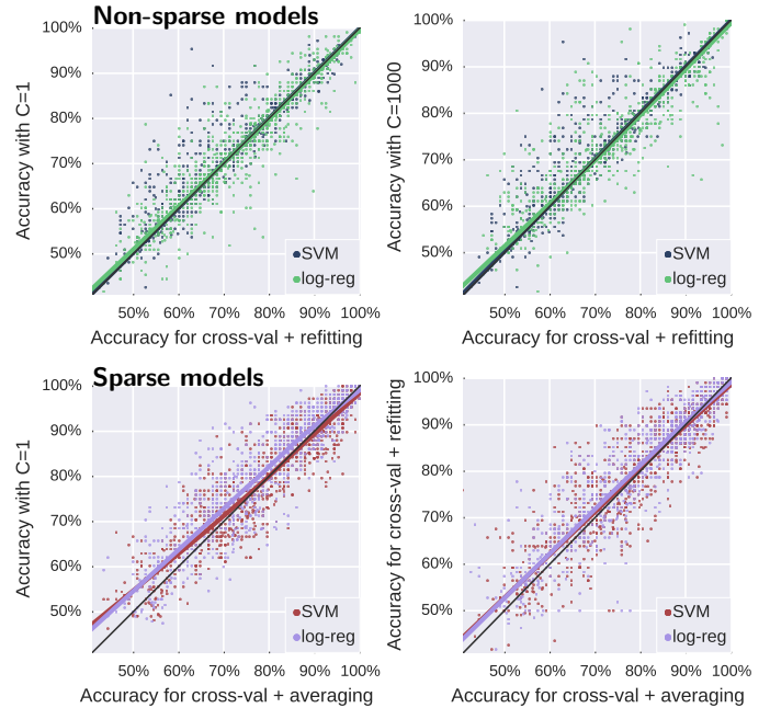
Figure A3: Comparing parameter-tuning strategies on prediction accuracy. Relating pairs of tuning strategies. Each dot corresponds to a given dataset, task, and validation split. The line is an indication of the tendency, using a lowess non-parametric local regression. The top row summarizes results for non-sparse models, SVM \ell_2 and logistic regression \ell_2 ; while the bottom row gives results for sparse models, SVM \ell_1 and logistic regression \ell_1 .
