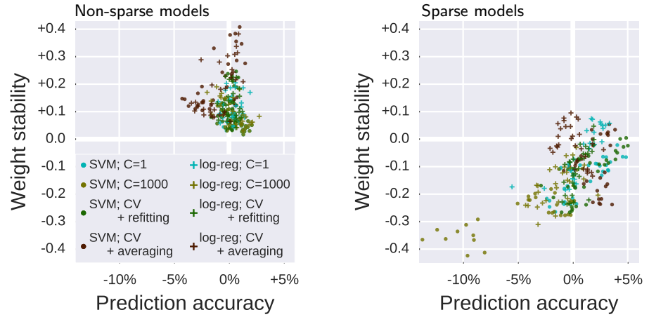
Figure A7: Prediction – stability tradeoff This figure gives the data points behind 11, reporting the stability of the weights, relative to the split’s average, as a function of the delta in prediction accuracy. Each point corresponds to a specific prediction task in our study.
