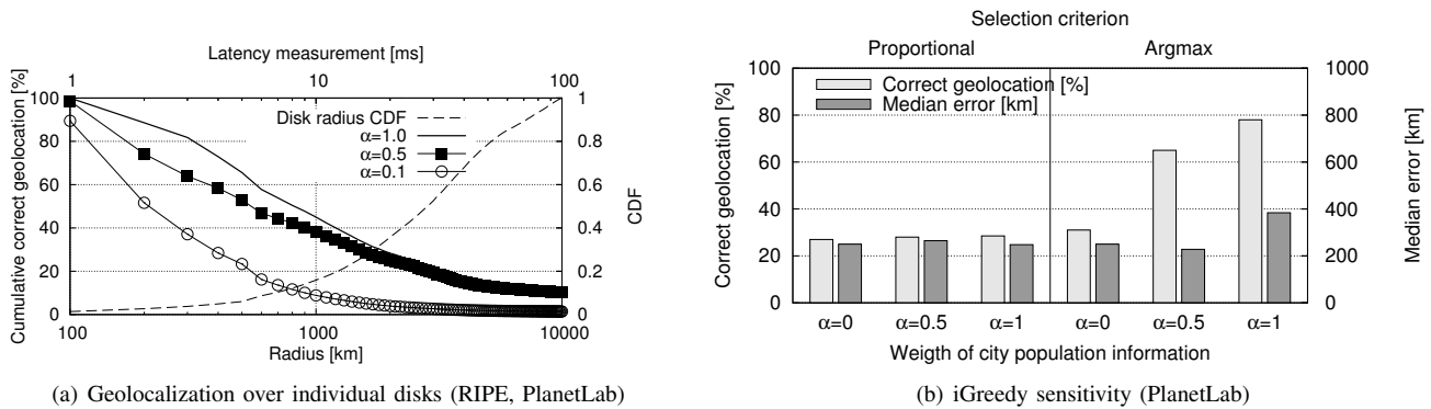
Fig. 5. Tuning iGreedy classification: (a) cumulative true positive geolocalization over all disks, with argmax selection for different weighting factor \alpha . (b) iGreedy performance for different selection policies and weighting factor settings.
