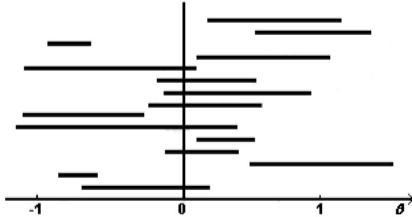
Figure 1: 50% confidence interval
