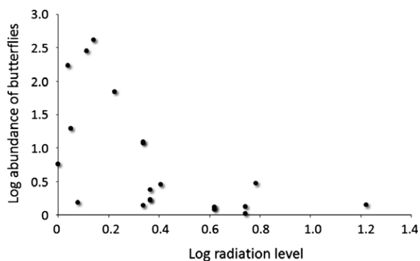
Fig. 3 Butterfly abundance plotted against radiation level ( \mu\text{Gy}/\text{h} ), both log-transformed.
