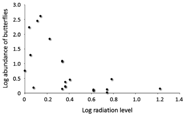
Fig. 3 Butterfly abundance plotted against radiation level ( \mu\text{Gy/h} ), both log-transformed.
