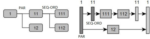
Figure 2: Set-up-lab example of an ACTIVITY-DL tasks-tree represented as a task tree on the left (a) and a work-flow on the right (b).
