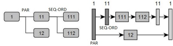
Figure 2: Set-up-lab example of an ACTIVITY-DL tasks-tree represented as a task tree on the left (a) and a work-flow on the right (b).
