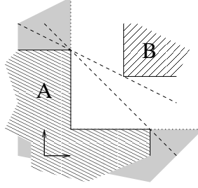
Figure 1: Binary interpolation in linear arithmetic. The hashed areas represent A and B (Eq. 28) respectively. A possible interpolant I between A and B ( A \Rightarrow I , I \Rightarrow \neg B ) is the grey area x \leq 1 \vee y \leq 1 . The dashed lines define two other possible interpolants, x + y \leq 5 and x + 2y \leq 9 .
