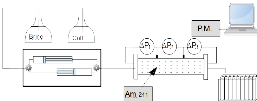
Figure 1 - Experimental setup.
