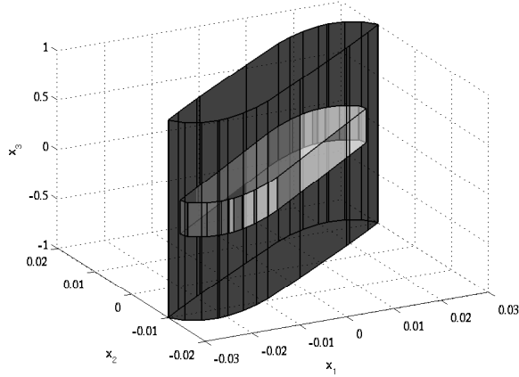
Figure 1: Polytopes \mathcal{S}_0 and \mathcal{S}_1 computed by Algorithm 1 using parameter setup C for system (20) with \underline{T} = 0.1 and \overline{T} = 0.5 ; \mathcal{S}_1 is strictly included in \mathcal{S}_0 .
