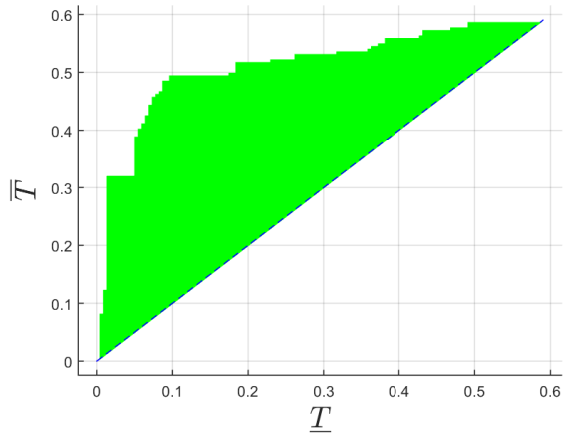
Figure 2: Timing contract synthesis for system (20): region \mathcal{T}^* of timing contract parameters, for which stability is guaranteed.
