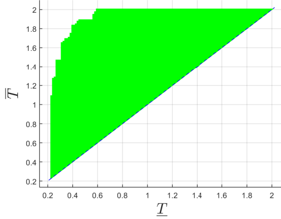
Figure 3: Timing contract synthesis for System (24) in the (\underline{T}, \overline{T}) domain.
