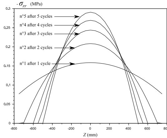
Figure 15: Contact pressure, -\sigma_{rr} for the last wrap
