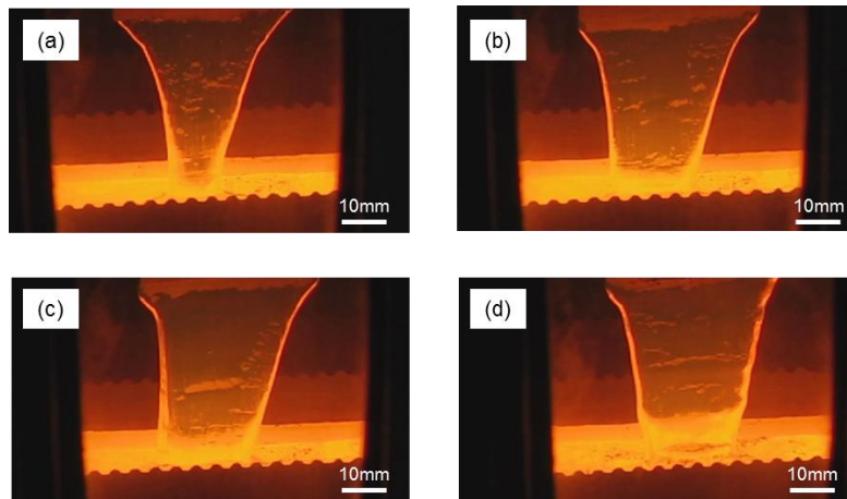
Fig. 2: Effect of applied various magnetic flux densities on the width of ribbon crystals (seed width=40 mm, seed thickness=300 \mu\text{m} , pulling rate=240 \mu\text{m/s} ): (a) 0 mT (b) 21.6 mT (c) 35.6 mT (d) 57 mT
