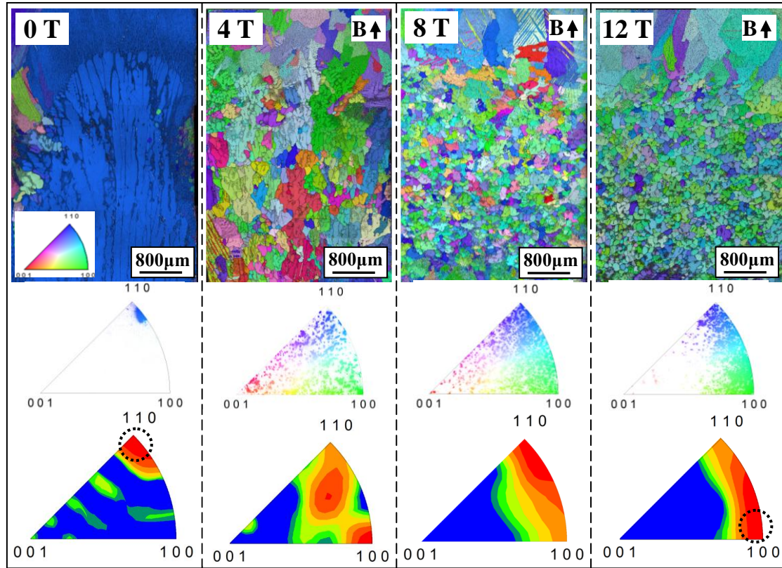
Fig. 2. EBSD orientation maps and corresponding pole figures for the structure near the liquid/solid interface in directionally solidified Sn-20wt%Pb alloy at a growth speed of 1 \mu\text{m/s} under various magnetic fields.
