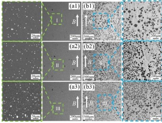
Fig. 1: BSE pictures of longitudinal microstructures of Bi-0.98Zn and Bi-0.44Zn under 29 T. a1-a3) are microstructures at the top, middle and bottom of Bi-0.98Zn alloy. b1-b3) are microstructures at the top, middle and bottom of Bi-0.44Zn alloy respectively
