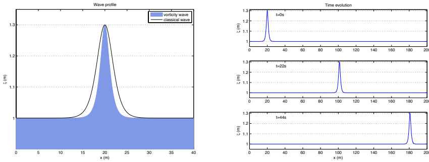
FIG. 4.2. Case E_\infty > 0 , v_\infty > 0 , F_\infty = 0 - Right-going wave with \varepsilon = 0.3 : initial profile (on the left) and snapshots at different locations along the channel (on the right).
