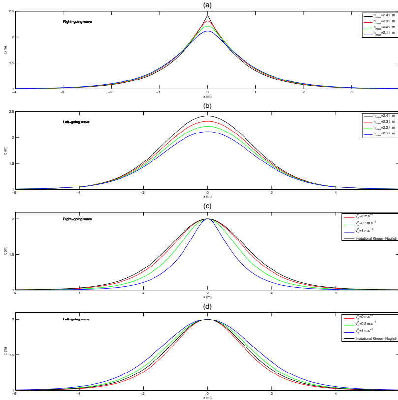
FIG. 2.2. Influence of v_\infty^\# > 0 on the profiles for H_0 = 1 m, E_\infty = 1 m 3 .s -2 and F_\infty = 0 . (a) Right-going solitary waves of nearly critical amplitudes for v_\infty^\# = 1 m.s -1 and therefore h_{\text{crit}} \approx 2.42 m. (b) Left going solitary waves for the same amplitudes. (c) Right-going solitary waves for h_{\text{max}} = 2 m and increasing values of v_\infty^\# . (d) Left-going solitary waves for h_{\text{max}} = 2 m and increasing values of v_\infty^\# .
