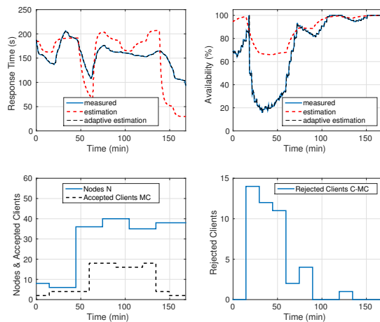
Figure 1: Comparison of adaptive and classic modeling
