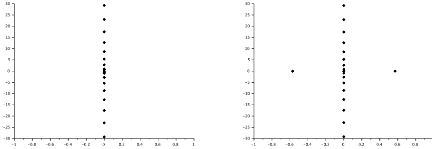
FIGURE 5.1. \sigma(J\mathcal{L}^{cn}) (left) and \sigma(J\mathcal{L}^{dn}) (right) on P_{4K} for k = 0.95
