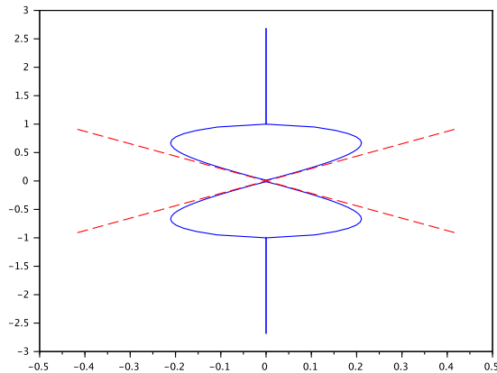
FIGURE 5.2. \sigma(J\mathcal{L}^{cn}) on L^2(\mathbb{R}) for k = 0.9 (plain (blue) curve), first order asymptotic around 0 (dashed (red) lines)
