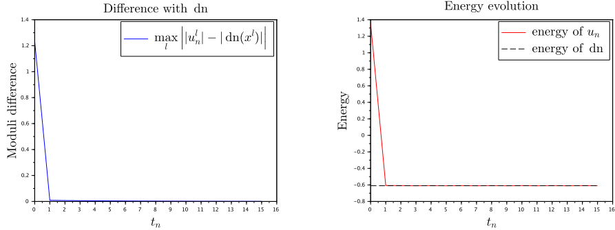
FIGURE 7.2. For m = \mathcal{M}(\text{dn}) = E(k) , focusing, periodic case
