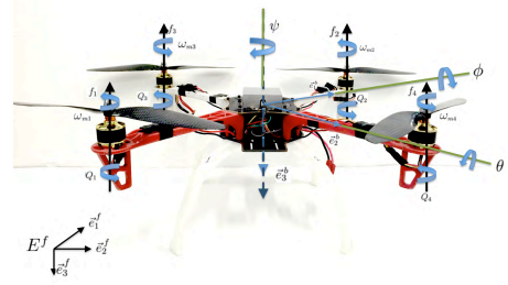
Fig. 4. Quadrotor: fixed frame \mathbf{E}^f = [\vec{e}_1^f, \vec{e}_2^f, \vec{e}_3^f] and body-fixed frame \mathbf{E}^b = [\vec{e}_1^b, \vec{e}_2^b, \vec{e}_3^b]
