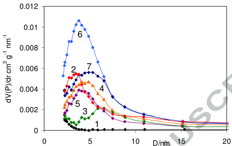
Fig. 2. Mesopore size distributions from N 2 adsorption isotherms at 77°K for parent wheat straw (1) and organosolv residues from treatments with H 2 SO 4 (2), FeCl 2 (3), CuCl 2 (4), FeCl 3 (5), Ga(OTf) 3 (6), Sc(OTf) 3 (7).
