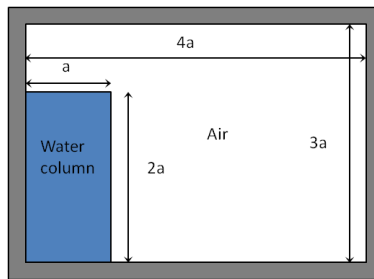
Figure 9: Collapse of water column [19, 24]
