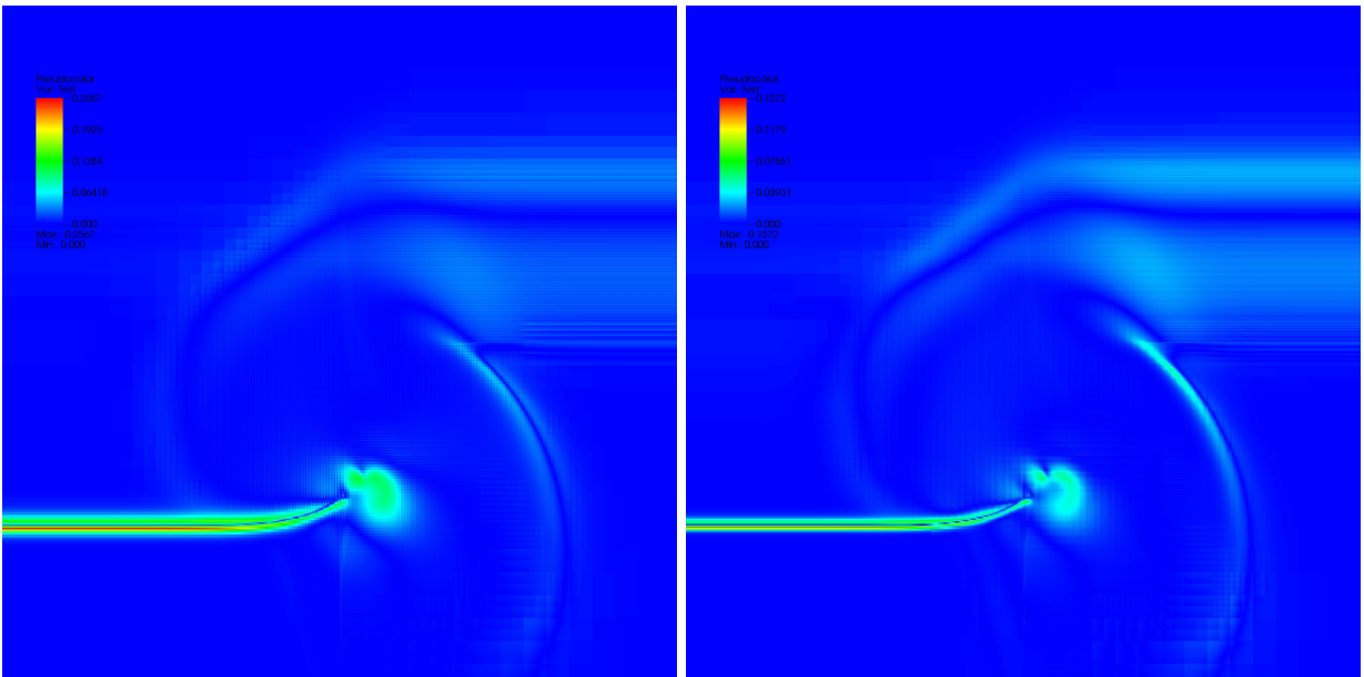
(c) L_{max} = 3 .
