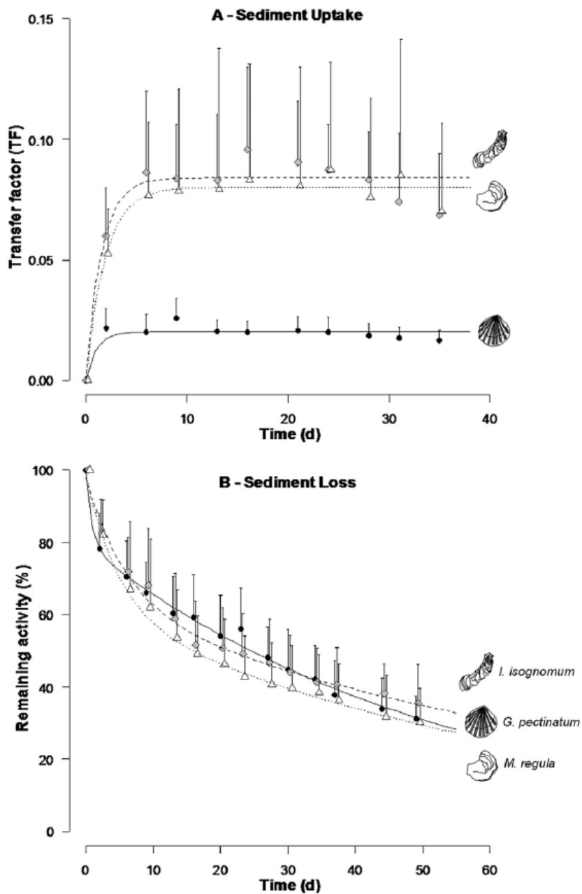
Figure 4. Uptake kinetics (A) of Cs in three bivalve's species ( G. pectinatum , I. isognomum and M. regula ) exposed for 35 d to the radiolabelled sediments (n = 10-20) and their following depuration kinetics (B) when thereafter maintained for 49 d in clean sediment and seawater (n = 7-15). All values are mean + SD and equations of kinetic model are described in Table 2.
