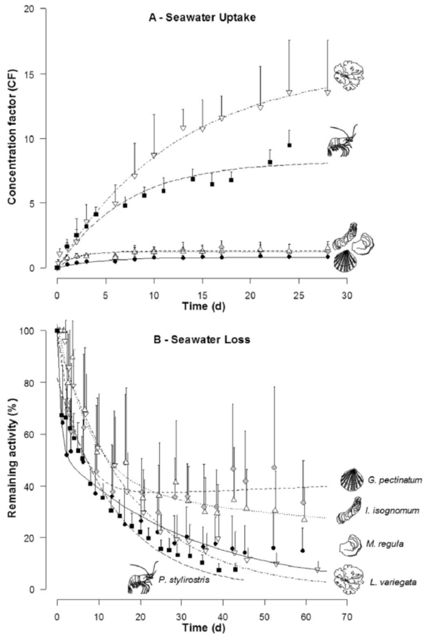
Figure 1. Uptake kinetics (A) of Cs in three bivalve's species ( G. pectinatum , I. isognomum and M. regula ), one species of shrimp ( P. stylirostris ) and one alga ( L. variegata ) for 24-28 d to dissolved radiotracers (n = 10-22) and their following depuration kinetics (B) when thereafter maintained for 43-62 d in clean seawater (n = 7-15). All values are mean + SD and equations of kinetic models are described in Table 2.
