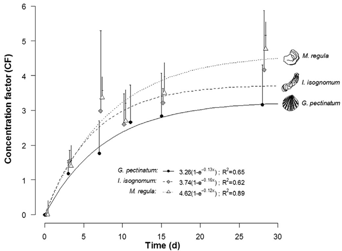
Figure 2. Whole soft-parts Concentration Factors (CF, mean \pm SD, n = 3-5) of ^{134}\text{Cs} in three bivalve species ( G. pectinatum , I. isognomum and M. regula ) during seawater experiment (28 d-exposure).
