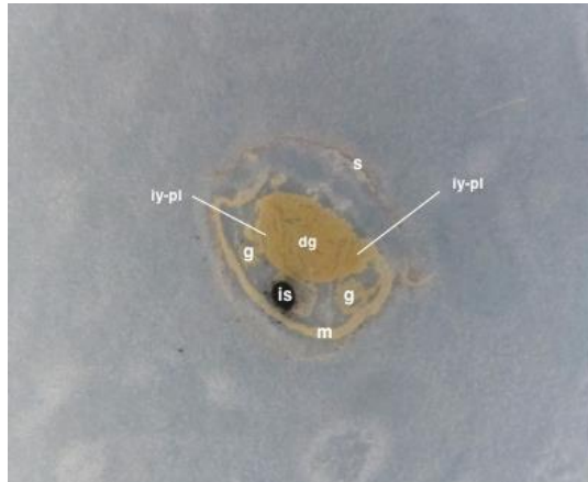
Figure 4. Cross body section (left) and autoradiogram (right) of a newly hatched juvenile of Sepia officinalis after exposure to dissolved ^{110m}\text{Ag} during the last week of embryonic development: dg: digestive gland, g: gills, is: ink sac, iy-pl: posterior lobes of the inner yolk sac (see Boletzky, 2002), m: muscle, s: skin. Note that the ^{110m}\text{Ag} is mainly found in gills and inner yolk sac suggesting that embryo accumulates Ag both directly from seawater and from vitelline reserve.
