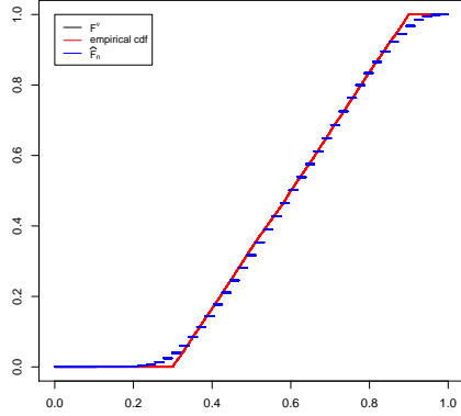
Figure 5: U(0.3, 0.9) : n = 10000 , T_n = 106714 , \widehat{M}_n = 46 , N_\infty \approx 0.068 .
