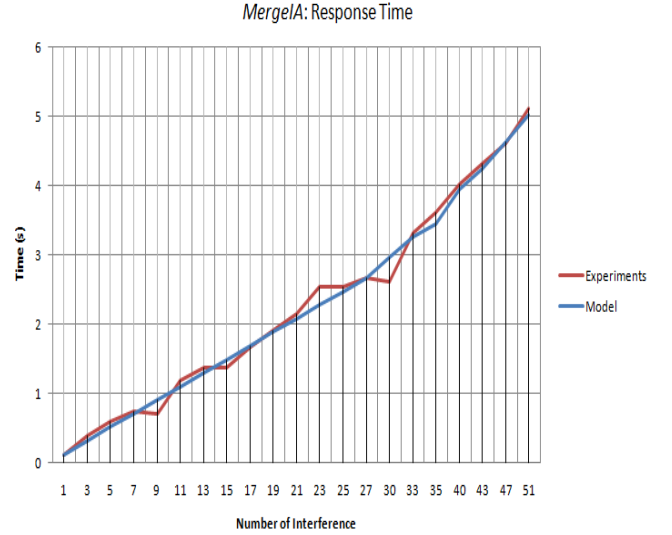
Figure 6. MergeIA: Response Time according to number of interference
