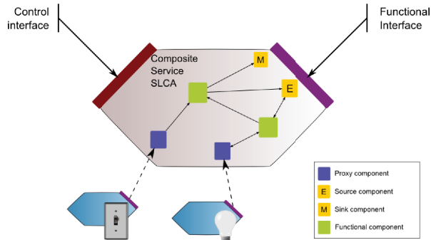
Fig. 7. Composite web service with evented communications
