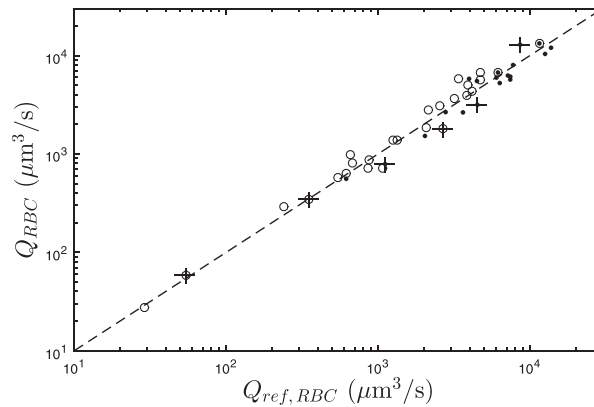
FIG. 5. RBC flow rate obtained from Equation (4) as a function of a reference RBC flow rate value obtained by counting. Circles: measurements in 10 \mu\text{m} \times 10 \mu\text{m} microchannels; Dots: measurements in 20 \mu\text{m} \times 20 \mu\text{m} microchannels; Dashed line: identity function. The error bars are shown for a limited set of data points only, for sake of clarity. The error bars on Q_{ref,RBC} come from the RBC-counting error and are \pm 0.15 \times Q_{ref,RBC} . The error bars on Q_{RBC} are mainly caused by experimental errors on the determination of V_0 and H_t , see Equation (4) and are \pm 0.17 \times Q_{RBC} .
