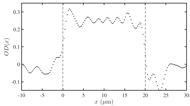
FIG. 2. Typical optical density profile OD(x) , obtained from an image sequence of RBC flowing in a 20 \mu\text{m} \times 20 \mu\text{m} micro-channel. The vertical dotted lines indicate the location of the microchannel walls.
