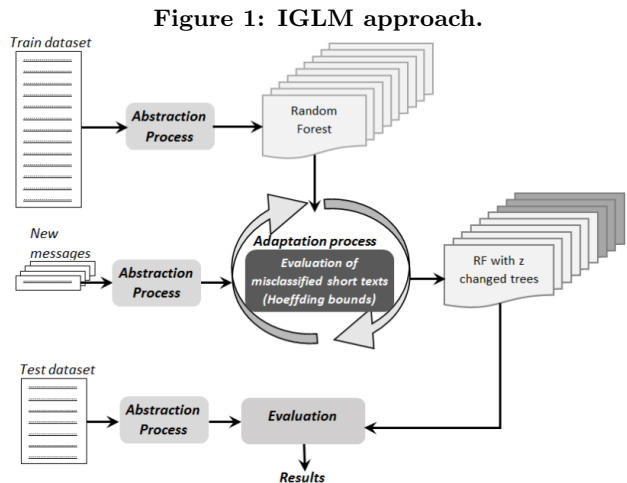
Figure 1: IGLM approach.
