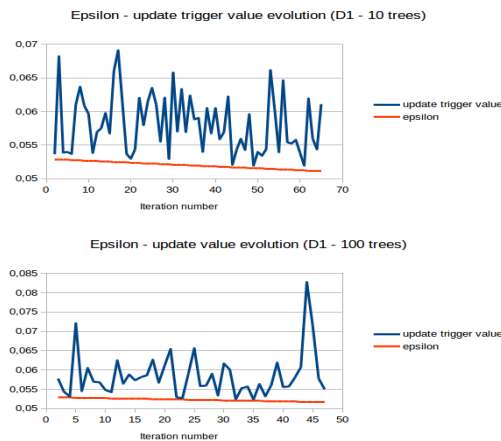
Figure 5: Epsilon - Update value evolution
