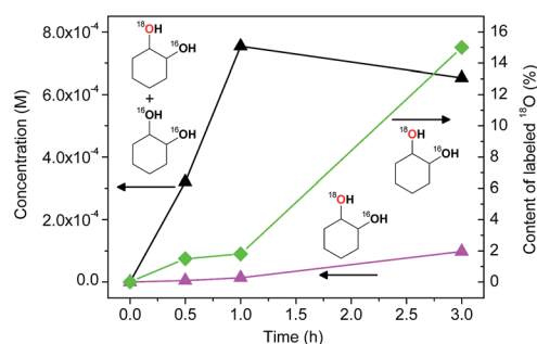
Fig. 20 Kinetic curves of accumulation with time of 1,2-cyclohexanediol containing both partially labeled (the sum 16 O + 18 O) and completely 18 O-labeled oxygenates (left Y-axis). Incorporation of the labeled oxygen into the 1,2-cyclohexanediol in the course of the cyclohexane oxidations is also shown (right Y-axis). Conditions: [I] 0 = 2 × 10 −4 M; [HNO 3 ] 0 = 0.05 M; [H 2 O 2 ] 0 = 0.91 M; [cyclohexane] 0 = 0.48 M; 30 °C; [H 2 18 O] 0 = 2.15 M. The yields and isotopic abundances were measured after reduction of the reaction samples with PPh 3 .
