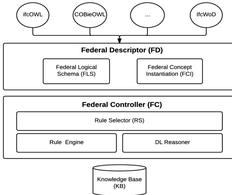
Figure 1. FOWLA architecture applied for AEC ontologies.
