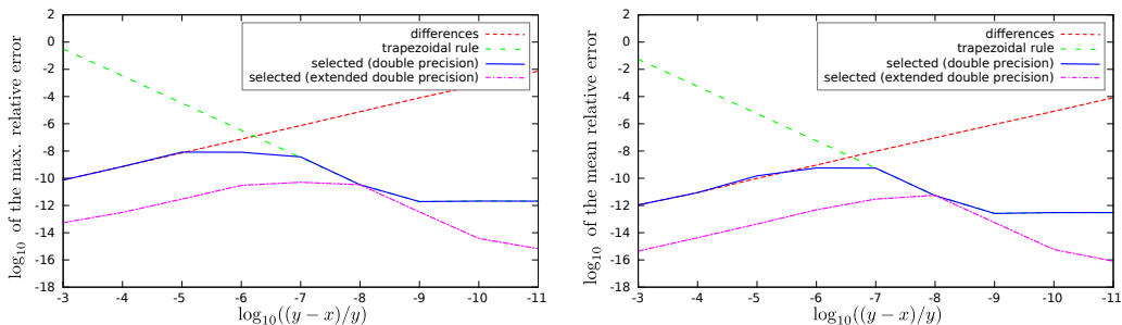
Figure 5: Control of maximum and mean relative errors associated to the computation of I_{x,y}^{\mu,p} using differences or a first order trapezoidal rule. In Section 3.2, we proposed to approximate the integral I_{x,y}^{\mu,p} by a difference of generalized incomplete gamma functions, I_{x,y}^{\mu,p} \approx I_{\text{diff}} = A - B (see Table 1 to derive the values of A and B according to x, y, \mu, p ), or using a trapezoidal rule, I_{x,y}^{\mu,p} \approx I_{\text{trapezoid}} . We proposed in Section 3.3 an explicit criterion, based on the computation of a ratio of (some estimates of) the absolute errors |\Delta I_{\text{diff}}| and |\Delta I_{\text{trapezoid}}| associated to those two approximations, which can be used to automatically select which approximation should be used. For several values of \delta_r = (y-x)/y , we computed I_{x,y}^{\mu,p} for a large range of parameters ( \mu = \pm 1 , p integer in [1, 1000] , y integer in [1, 1000] , and x being the floating-point number closest to y(1 - \delta_r) ). We display here the evolution, as a function of \log_{10}(\delta_r) , of the maximal (left-side) and mean (right-side) relative error observed when using the approximation by differences I_{\text{diff}} (dashed red curve, standard double precision implementation), or when using the approximation by trapezoidal rule I_{\text{trapezoid}} (dashed green curve, standard double precision implementation), or when automatically selecting the computation method (plain blue curve for the standard double precision implementation, dotted purple curve for the extended double precision implementation), thanks to the criterion proposed in Section 3.3. We see that the plain blue curve lies almost everywhere below the dashed curves, showing that the criterion efficiently selects the best accurate approximation. We can see also that the error can be improved by three orders of magnitude using extended double precision, except when \delta_r \approx 10^{-8} (in that case, the precision is limited by the fact that we only use one term in the trapezoidal rule).
