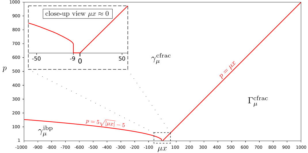
Figure 4: Numerical evaluation of the generalized lower or upper incomplete gamma functions. In this figure, we display the graph (red curve) of the frontier p_{\text{lim}} defined in (24). This curve delimits the plan (\mu x, p) into three regions, each corresponding to the region where one of the three computation methods \gamma_{\mu}^{\text{frac}} , \gamma_{\mu}^{\text{ibp}} and \Gamma_{\mu}^{\text{frac}} is optimal (in the sense that its computation is fast and reaches a good relative error). According to our partition, and as indicated on the figure, \gamma_{\mu}^{\text{ibp}} must be computed in the bottom-left region, \gamma_{\mu}^{\text{frac}} in the middle region, and \Gamma_{\mu}^{\text{frac}} in the bottom-right region. More precisely, we select \gamma_{\mu}(p, x) as soon as p \geq p_{\text{lim}}(\mu x) , otherwise we select \gamma_{\mu}^{\text{ibp}}(p, x) when \mu < 0 , or \Gamma_{\mu}^{\text{frac}}(p, x) when \mu > 0 . A close-up view near \mu x = 0 shows that \gamma_{\mu}^{\text{frac}} is automatically selected near \mu x = 0 since p \geq 1 \geq p_{\text{lim}}(\mu x) = 0 when -9 \leq \mu x \leq 0 (this avoids the computation of \gamma_{\mu}^{\text{ibp}}(p, x) for |\mu x| < \max(1, p-1) , which is not allowed according to the discussion of Section 2.1.3).
