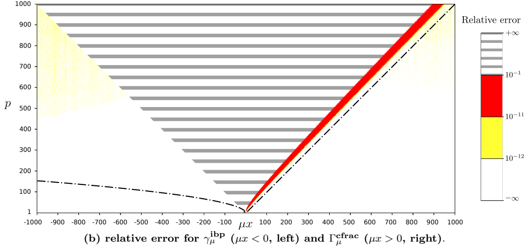
Figure 2: Control of the relative error associated to the computation of \gamma_\mu(p, x) and \Gamma_\mu(p, x) using different methods. We used Algorithms 3 and 4 (implemented in C language, using the standard double datatype on a 64-bits computer) to compute \gamma_\mu^{\text{frac}}(p, x) , \gamma_\mu^{\text{ibp}}(p, x) , \Gamma_\mu^{\text{frac}}(p, x) for \mu = \pm 1 , x integer in [0, 10^3] , and p integer in [1, 10^3] . Using Maple, we measured the relative errors reached by each method. The error reached by \gamma_\mu^{\text{frac}} is displayed in (a), the error reached by \gamma_\mu^{\text{ibp}} (computed only for \mu < 0 and |\mu x| \geq \max(1, p - 1) ) is displayed in the left-side of (b), and the error reached by \Gamma_\mu^{\text{frac}} (computed only for \mu > 0 ) is displayed in the right-side of (b). The dashed curve (see its parametric equation in (24)) splits the plan (\mu x, p) into three domains, each one is associated to one of the three computation methods ( \gamma_\mu^{\text{ibp}} : left, \gamma_\mu^{\text{frac}} : middle, \Gamma_\mu^{\text{frac}} : right), and corresponds to the region where the method is at the same time fast and accurate, compared to the others (see also Figure 4). We can see that inside each one of the three domains, the corresponding computation method reaches a relative error always less than 10^{-11} (the actual maximal observed error is in fact close to 2 \cdot 10^{-12} ), and most of the time less than 10^{-12} (in practice close to 10^{-13} ). We also observe that the boundary of the region where the relative error (of the selected algorithm) is greater than 10^{-12} coincides almost perfectly with the isovalue \sigma = 4503.5 displayed in Figure 1, showing that the relative error is in practice only limited by the mantissa-exponent representation (see discussion in Section 2.3). This limitation can be compensated by using a more precise floating-point representation, as shown in Figure 3.
