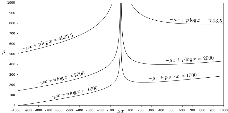
Figure 1: Isovalues of the exponent \sigma = (\mu, x, p) \mapsto -\mu x + p \log x ( \mu = -1 , left) and ( \mu = 1 , right). In this figure, we display some isovalues of the exponent part of \gamma_\mu and \Gamma_\mu computed with Algorithm 3 and 4, and whose parametric equation is recalled above. As discussed in Section 2.3, the relative precision related to the evaluation of \gamma_\mu and \Gamma_\mu using a mantissa-exponent representation \rho \cdot e^\sigma deteriorates as \sigma increases. Indeed, even when \rho and \sigma are estimated with the best available precision ( \Delta\rho/\rho = \Delta\sigma/\sigma = \varepsilon_{\text{machine}} ), the best relative precision that we can expect for the evaluation of \rho \cdot e^\sigma is E_{\min} = (1 + |\sigma|) \cdot \varepsilon_{\text{machine}} , as stated in (21). The standard precision (on a 64-bits computer) is \varepsilon_{\text{machine}} = 2.22 \cdot 10^{-16} , so that E_{\min} \geq 10^{-12} as soon as \sigma \geq 4503.5 . Interestingly enough, the curve corresponding to the isovalue \sigma(\mu, x, p) = 4503.5 fits particularly well with the frontier of the domain where Algorithm 3 and 4 yield a relative accuracy more than 10^{-12} (see Figure 2). When using the extended double floating-point precision (corresponding to the long double datatype in C language), we have \varepsilon_{\text{machine}} = 1.08 \cdot 10^{-19} , so that we get 1 \cdot 10^{-16} \leq E_{\min} \leq 2 \cdot 10^{-16} , in the region 1000 \leq \sigma(\mu, x, p) \leq 2000 (delimited by the two other isovalues represented above). Again, these two frontiers were experimentally observed in Figure 3, where we measure the relative error reached by our algorithms using extended double precision.
