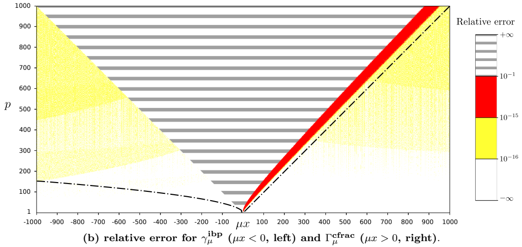
Figure 3: Improving the accuracy of \gamma_\mu(p, x) and \Gamma_\mu(p, x) using extended double precision. We performed here the same experiment as in Figure 2, using a C implementation of Algorithms 3 and 4 with extended double precision (corresponding to the long double datatype in C language, with machine epsilon \varepsilon_{\text{machine}} = 1.08 \cdot 10^{-19} , which is around three orders of magnitude better than the standard double precision). We see that our algorithm fully benefits from this additional precision, since the observed relative error is decreased of around three magnitude orders as well. Besides, we observe again that the main limitation to the precision remains that involved by the mantissa-exponent representation, since, within each domain, the level lines of the relative error of the selected algorithm match very well to the isovalues of \sigma , and the value of the relative error is in practice very similar to that predicted in (21). This suggests that the error bounds we obtain could be reduced even further by simply using a more precise floating-point arithmetic (for instance the GNU MPFR C library).
