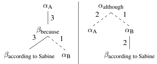
Figure 10: The derivation trees for A \text{ CONJ, according to Sabine, } B with a CConj (left) or a PConj (right).
