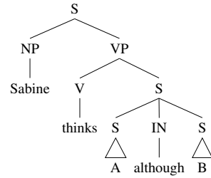
Figure 9: Syntactic derived trees for sentences of the form \text{Sabine thinks } A \text{ although } B . Note that with although (a PConj), the tree at the bottom corresponds to a less likely reading that must be forced by the context.
