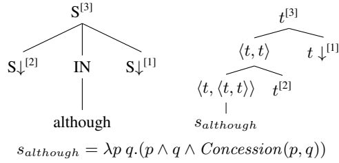
Figure 5: PConj: \alpha_{\text{although}}
