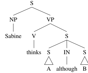
Figure 9: Syntactic derived trees for sentences of the form Sabine thinks A although B . Note that with although (a PConj), the tree at the bottom corresponds to a less likely reading that must be forced by the context.
