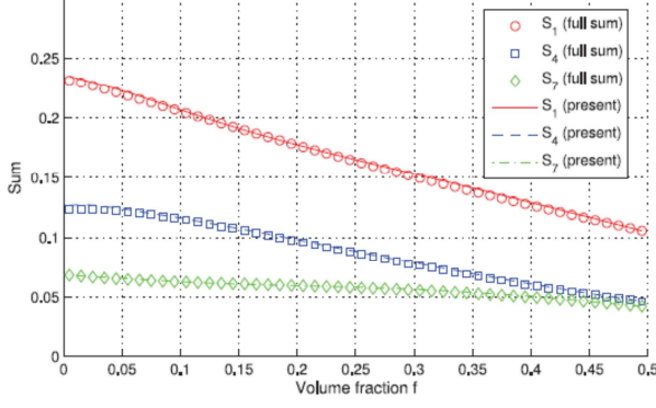
Fig. 4. Comparison between the full lattice sums with resolution -128 < n_i \leq 128 and Eqs. (67,68) for the FCO case. The spheroids and the unit cell have the same dimension ratio a \times a \times 0.5a and R \times R \times 0.5R . The cutoff radius is \eta'_c = 4\epsilon and \epsilon = 2\pi R/a . For the sake of clarity, only the sums S_1 , S_4 and S_7 are presented.
