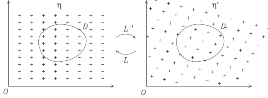
Fig. 1. Grid \eta and \eta' in Fourier space.
