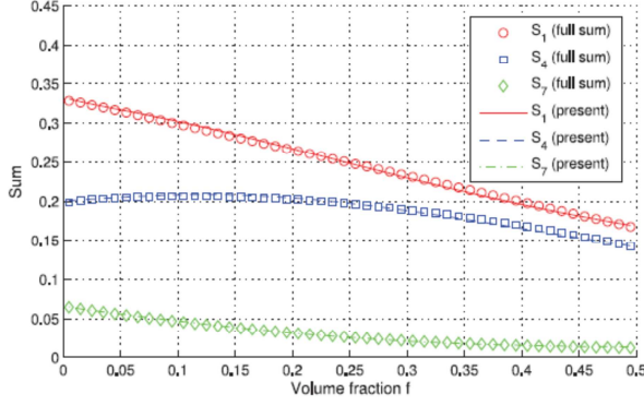
Fig. 3. Comparison between the full lattice sums with resolution -128 < n_i \leq 128 and Eq. (59) for the simple cubic case. At f = 0 , the lattice sums take the limit values S_1 = 1/3 , S_4 = 1/5 , and S_7 = 1/15 .
