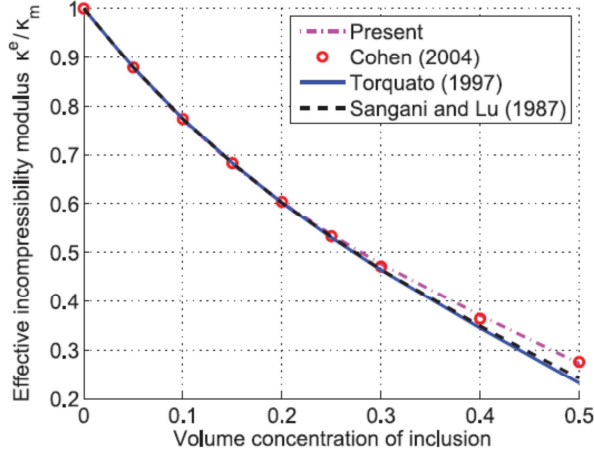
Fig. 6. Effective bulk modulus \kappa^e/\kappa_m for a simple cubic array of void spheres.
