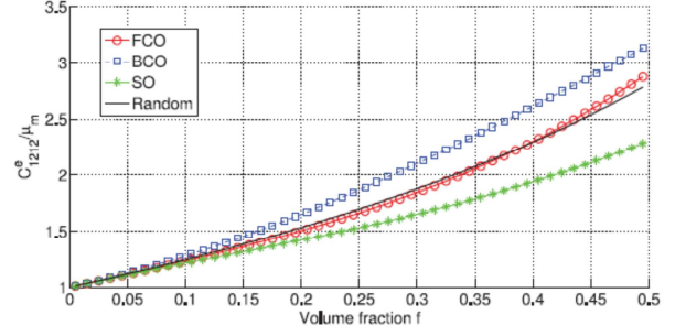
Fig. 8. Dimensionless effective shear moduli C_{1212}^e/\mu_m for FCO, BCO, SO, and random arrangements of spheroids.
