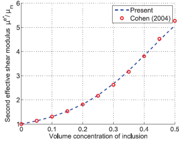
Fig. 7. Effective shear modulus \mu^e/\mu_m for a simple cubic array of rigid spheres.
