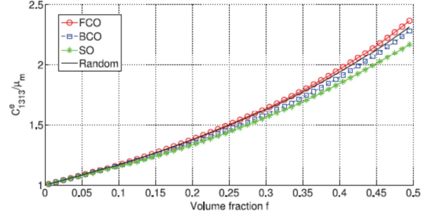
Fig. 9. Dimensionless effective shear moduli C_{1313}^e/\mu_m for FCO, BCO, SO, and random arrangements of spheroids.
