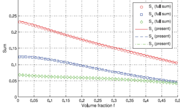
Fig. 4. Comparison between the full lattice sums with resolution -128 < n_i \leq 128 and Eqs. (67,68) for the FCO case. The spheroids and the unit cell have the same dimension ratio a \times a \times 0.5a and R \times R \times 0.5R . The cutoff radius is \eta'_c = 4\epsilon and \epsilon = 2\pi R/a . For the sake of clarity, only the sums S_1 , S_4 and S_7 are presented.
