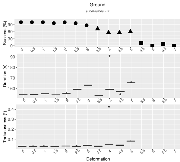
Fig. 9: Success rate, times, and tortuosity results for subdivision s = 2 and with no obstacle
