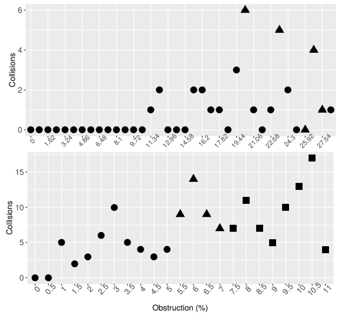
Fig. 12: Number of collisions. Top graph: for the buildings maps, bottom graph: for the trees maps
