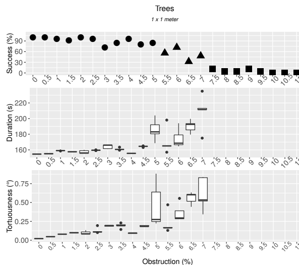
Fig. 7: Success rate, times, and tortuousness results for trees obstacles on a flat ground
