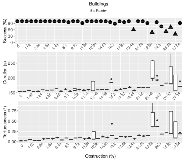
Fig. 8: Success rate, times, and tortuosity results for buildings obstacles on a flat ground
