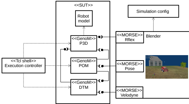
Fig. 1: Simplified diagram of the test architecture
