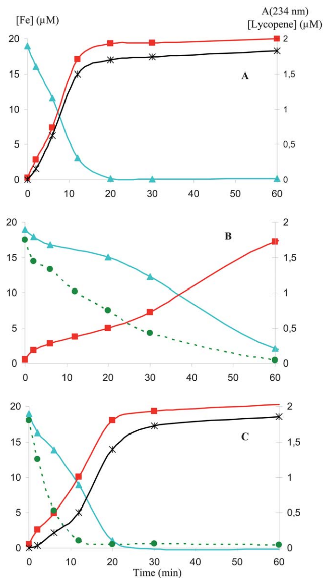
Fig. 4 Conversion of \text{Fe}^{\text{II}} (▲) into \text{Fe}^{\text{III}} (■) (left scale), conjugated diene accumulation (*) and lycopene consumption (dashed curve, ●) (right scale) in acetate buffer pH 4 + Brij®35, 37 °C. (A) \text{Fe}^{\text{II}} + linoleic acid, (B) \text{Fe}^{\text{II}} + lycopene, (C) \text{Fe}^{\text{II}} + linoleic acid + lycopene. Initial concentrations = 20 \mu\text{M} \text{Fe}^{\text{II}} , 0.7 mM linoleic acid, 2 \mu\text{M} lycopene.
