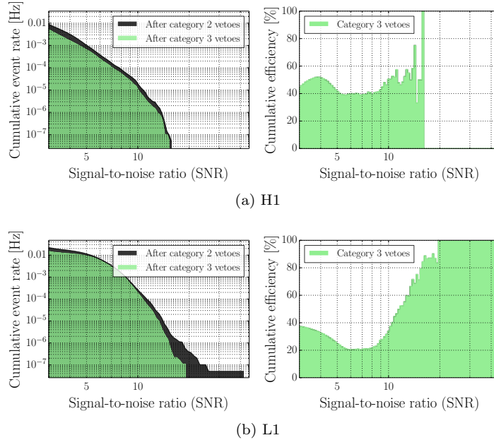
Figure 12: The effect of category 3 vetoes on the cWB pipeline for (a) H1 and (b) L1. The left panels show the reduction in event rate, while the right panels show the cumulative veto efficiency, both as a function of single-detector SNR.
