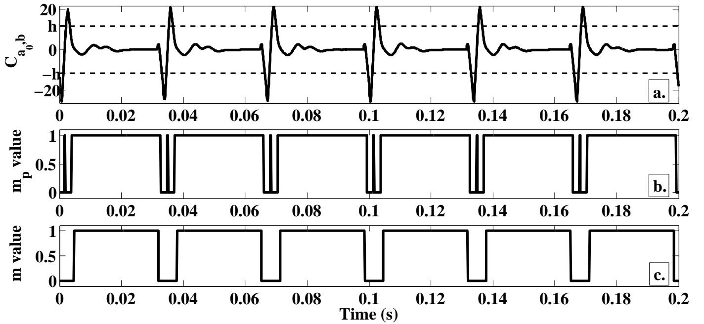
Fig. 3. Creation of mask removal example. a) C_{a_0, b} coefficients from CWT with a_0 scales factor. Both dash line are the h threshold representation for positive and negative parts computed with the equation 2. b). Preliminary m_p mask created with h threshold. c) Final m mask from an erosion on m_p .
