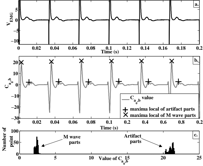
Figure 2: a) V_{EMG} signal example with an electrical stimulation at 30 Hz frequency, a 40 mA amplitude, 1 ms pulse time duration and a biphasic waveform performed on the right biceps muscle. b) CWT transformation for the V_{EMG} signal with a_0 = 38 corresponding to the maximum of C_{a,b} coefficient. Note the difference between maxima of C_{a,b} coefficients during artifacts (cross) and maxima C_{a,b} coefficients during M waves (plus) which allows the differentiation between artifacts and M waves. c) Histogram of local maxima values, showing a bimodal distribution.
