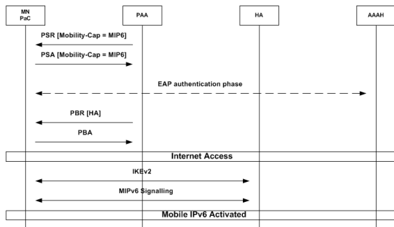
Fig. 5 MIP6 Bootstrapping with PANA: Exchanges
