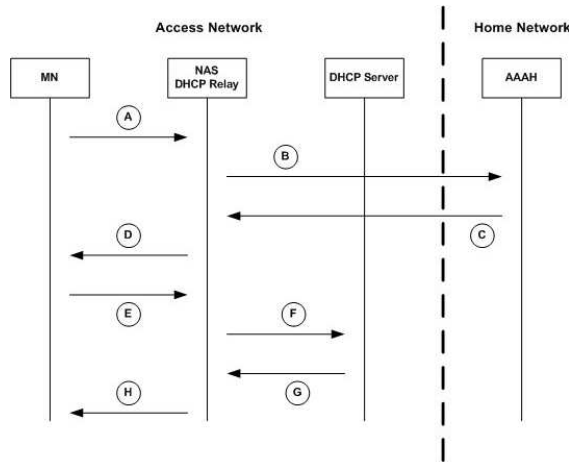
Fig. 3 MIP6 Bootstrapping with DHCPv6: Exchanges
