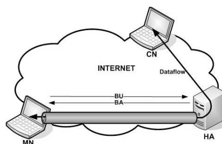
Fig. 1 Mobile IPv6 Architecture
