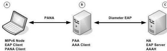
Fig. 6 PANA - Mobile IPv6 Testbed
