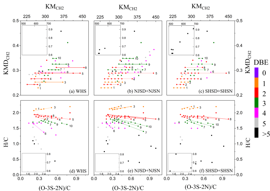
Figure 5. (a–c) CH 2 -Kendrick diagrams and (d–e) Van Krevelen diagrams for CHONS. The color-coding indicates the DBE values calculated from Eq. (1). The molecular formulas of the homologue series 1 to 10 can be written as C n H 2n+1 NO 3 SO 4 , C n H 2n-1 NO 3 SO 4 , C n H 2n+1 ONO 3 SO 4 , C n H 2n-1 ONO 3 SO 4 , C n H 2n-1 O 2 NO 3 SO 4 , C n H 2n-5 ONO 3 SO 4 , C n H 2n-3 O 2 NO 3 SO 4 , C n H 2n-1 O 3 NO 3 SO 4 , C n H 2n-3 O 3 NO 3 SO 4 , and C n H 2n-3 O 4 NO 3 SO 4 , respectively (n > 4).
