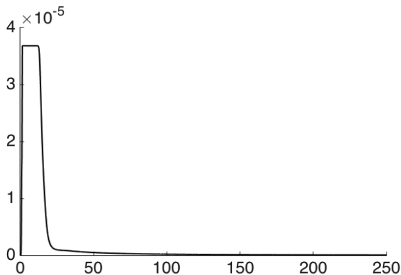
Figure 6 – the energy \mathcal{E}_e + \mathcal{E}_m defined by (2.20). As soon as the waves reach the PML, they are well absorbed and the energy is decaying, both for forward and backward waves.
