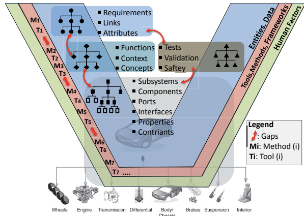
Figure 1: Part of the conceptual design entities context according to the V-model [6, 24]
