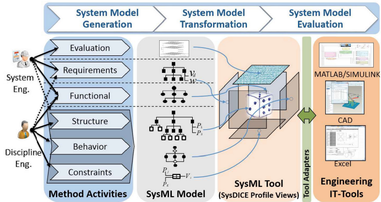
Figure 2: SysDICE overall framework
