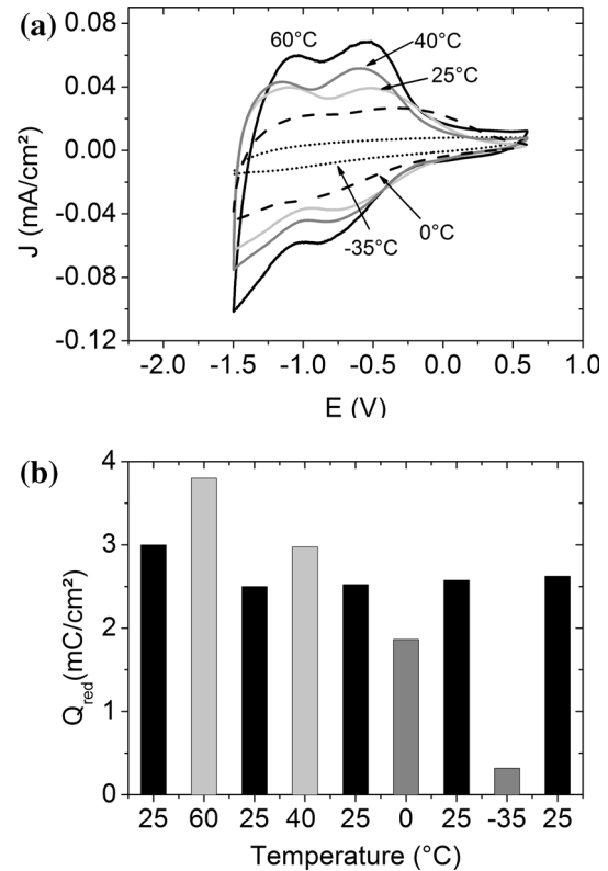
Fig. 9 CV of EC device \text{WO}_3/0.3 \text{ M LiTFSI BMITFSI} , 40 \% PMMA/ 2 \% \text{Ni}_{1-x}\text{O} at various temperatures (a) and histograms of the capacity versus temperature (b)
