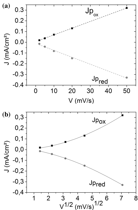
Fig. 5 Evolutions of J_{p_{ox}} and J_{p_{red}} of 2% Ni_{1-x}O thin films cycled in Pt/0.3 M LiTFSI in BMITFSI/ Ni_{1-x}O versus SCE versus scan rate of 2 to 50 mV/s (a) and versus square root of scan rate (b)
