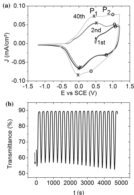
Fig. 6 CVs for 2% Ni_{1-x}O thin films cycled in Pt/0.3 M LiTFSI in BMITFSI/ Ni_{1-x}O versus SCE, start in oxidation using a scan rate of 20 mV/s and -1.2 to 1.2 V voltage window (a). In situ measurement of transmittance during chronoamperometry operate at -1.2 V(20 s)/1.2 V(20 s) (b)
