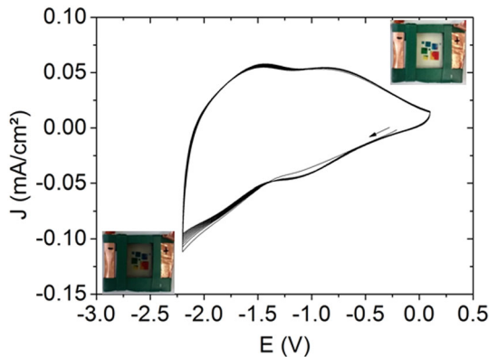
Fig. 7 CV of EC device \text{WO}_3/0.3 \text{ M LiTFSI BMITFSI} , 40 \% PMMA/ 2 \% \text{Ni}_{1-x}\text{O} . The visual appearances of the device in the bleached and colored states are also added
