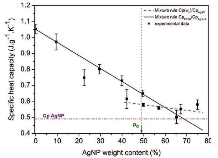
Fig. 2. Evolution of the specific heat capacity of the composites with silver nanoparticles weight content at 17 °C. Measured specific heat capacity (■), C_{p,PEEK} (— · — · —), C_{p,AgNP} (— · — · —), mixture rule C_{p,PEEK}/C_{p,Ag bulk} (—), mixture rule C_p(w_c)/C_{p,AgNP} (---). p_c is the electrical percolation threshold.
