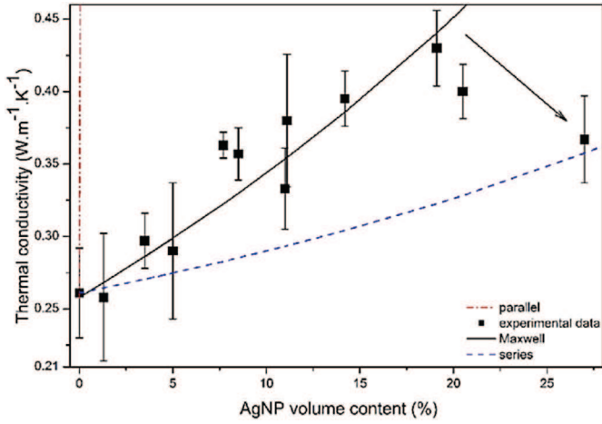
Fig. 4. Evolution of the thermal conductivity of the composites with silver nanoparticles volume content. Measured thermal conductivity at 17 °C (■), Maxwell model (—), Parallel model (— · —), Series model (---).
