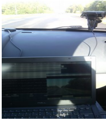
Figure 1. Simple experimental setup : linux-based acquisition computer, Usb Gps module (upper-left), Carl Zeiss Hd1080 camera (upper-right).
