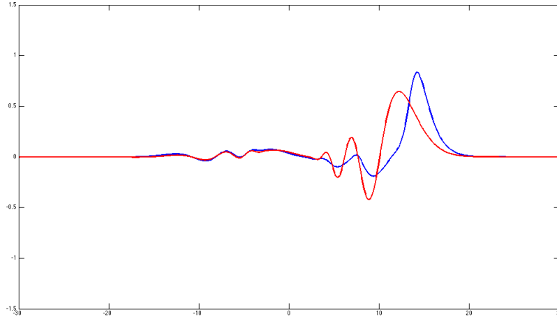
FIGURE 4. Evolution of the free surface for \varepsilon = 0 (red) and \varepsilon = 0.1 (blue).
