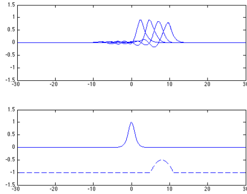
FIGURE 2. Upper: Evolution of the free surface for different times. Lower: bottom topography and initial condition.
