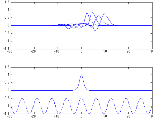
FIGURE 1. Upper: Evolution of the free surface for different times. Lower: bottom topography and initial condition.
