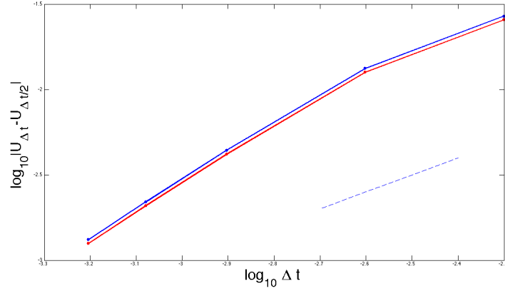
FIGURE 3. Convergence curve for the Lie method for two bottoms: bump (red line) and ripple bottom (blue line).
